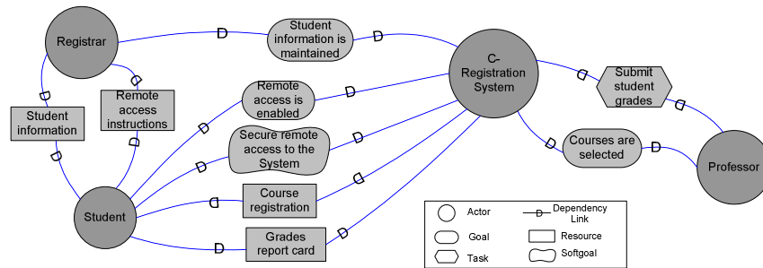
Fig.2. Excerpt of an i* model for the C-Registration System
